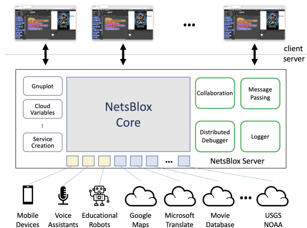
Fig. 8: NetsBlox architecture
